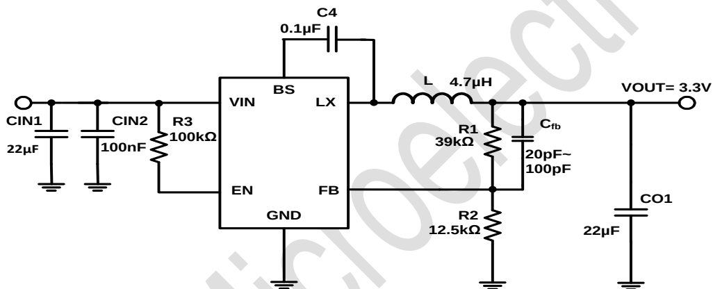
Figure 5. 12V IN , 3.3V Output ( V_{FB}=0.8V )
